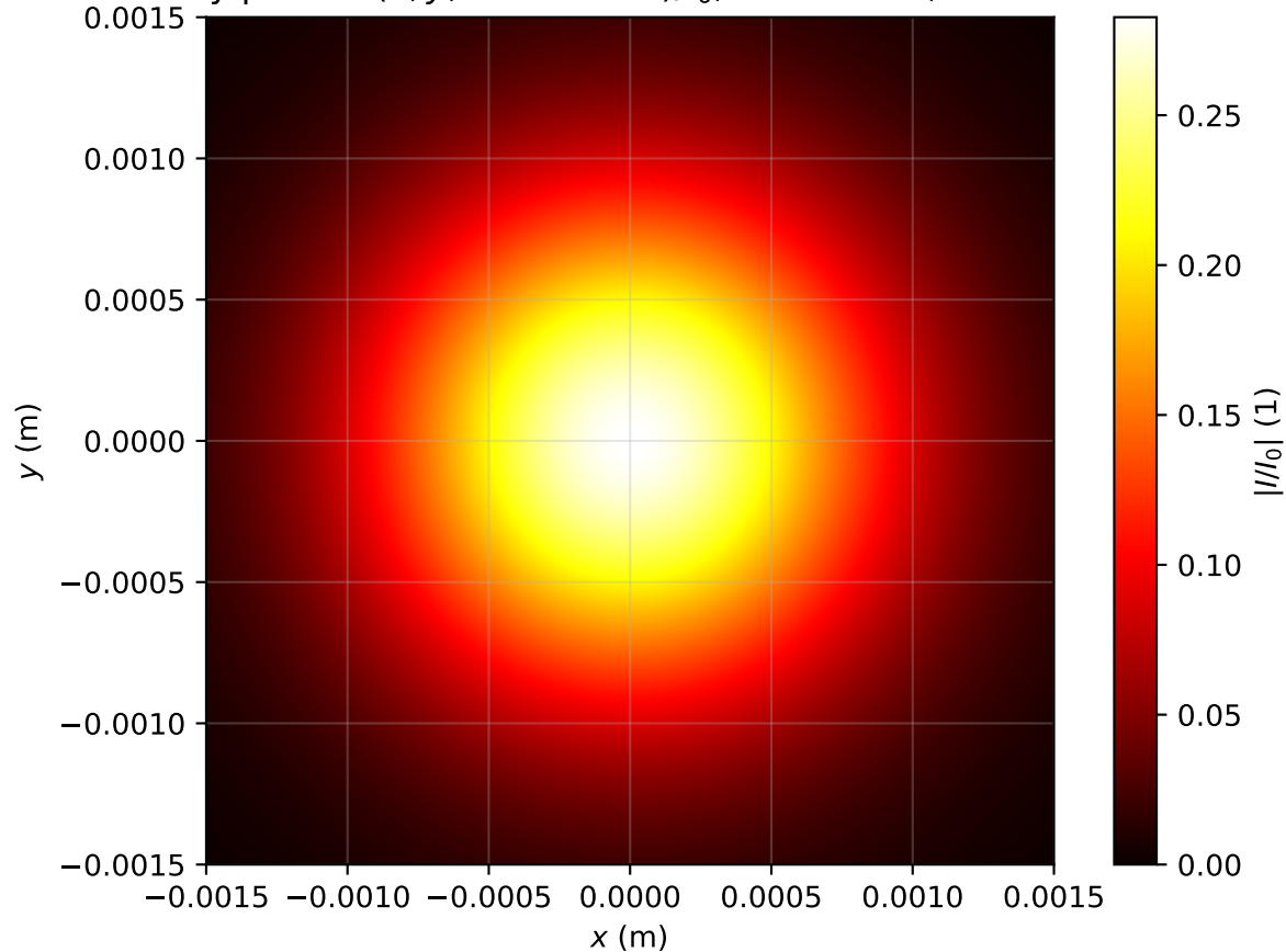
Intensity profile I(x, y, z = 3.662m)/I_0 , P_{in}=0.2P_{cr} , artificial time
